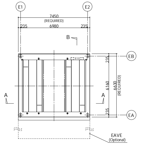
UPPER FLOOR PLAN S = 1/100
