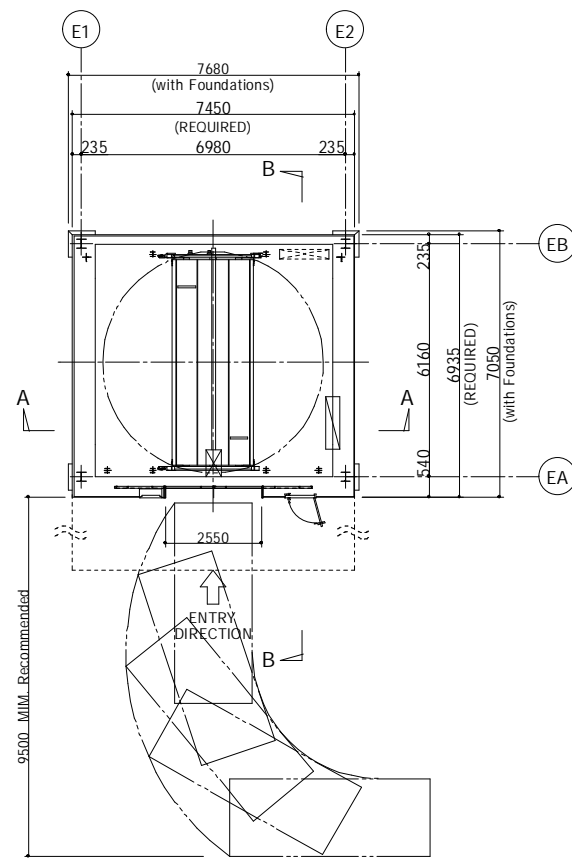
ENTRANCE-FLOOR (EL) LAYOUT PLAN S = 1/100
