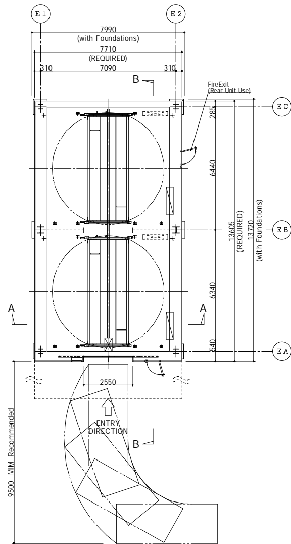
ENTRANCE-FLOOR (EL) LAYOUT PLAN S = 1/100
