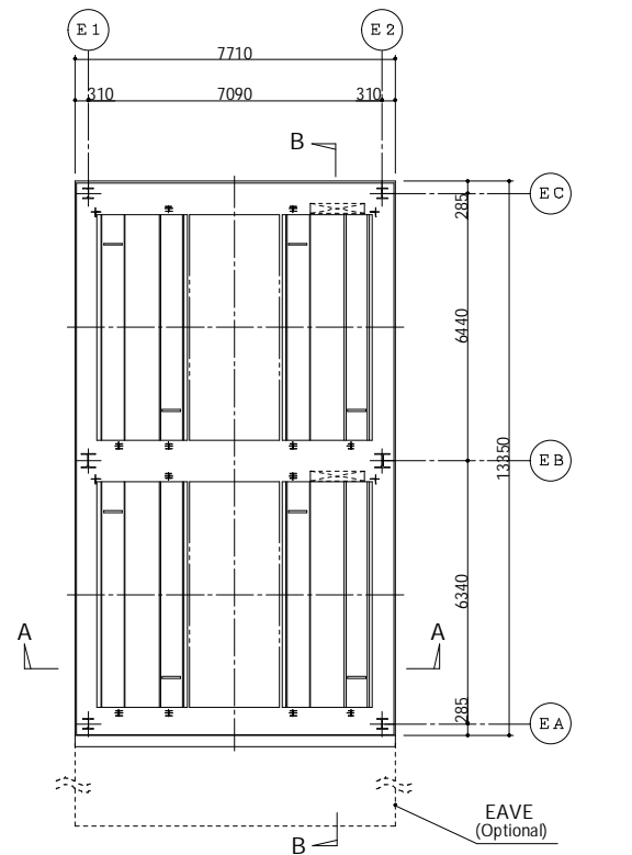
UPPER FLOOR PLAN S = 1/100
