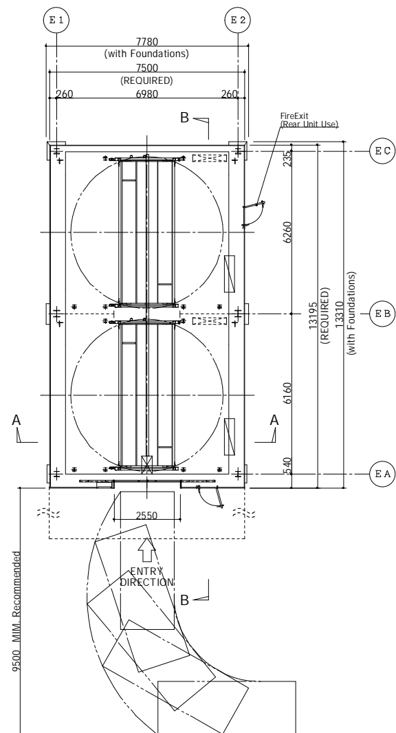
ENTRANCE-FLOOR (EL)LAYOUT PLAN S = 1/100
