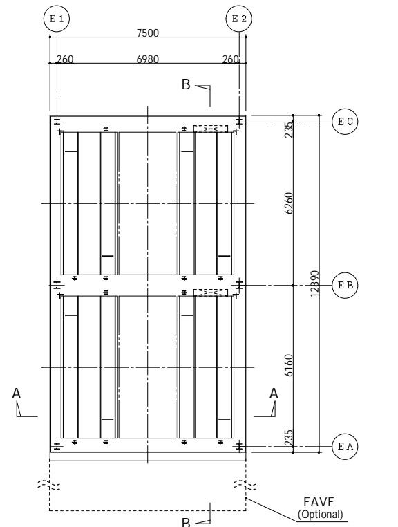
UPPER FLOOR PLAN S = 1/100
