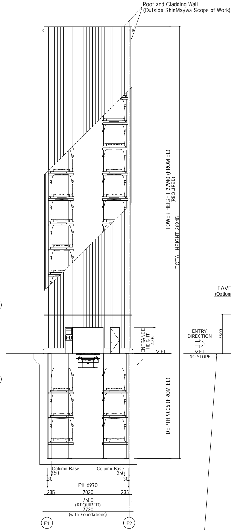
A-A SECTION S = 1/100
