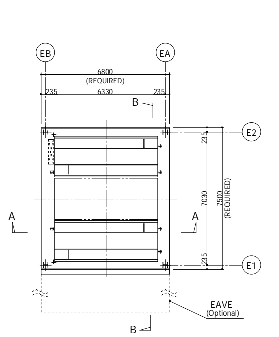
UPPER FLOOR PLAN S = 1/100
