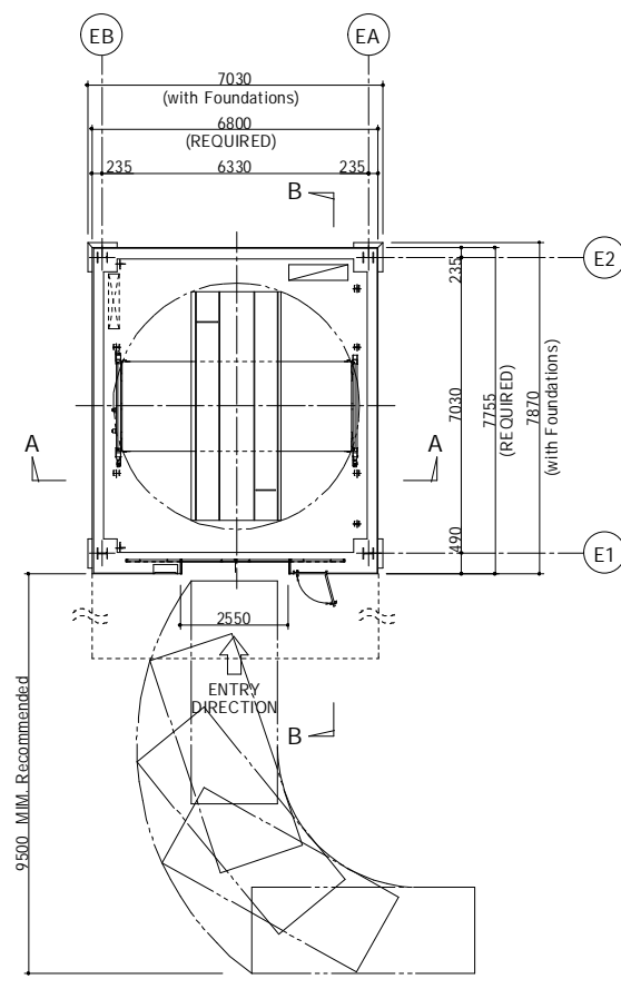
ENTRANCE-FLOOR (EL) LAYOUT PLAN S = 1/100
