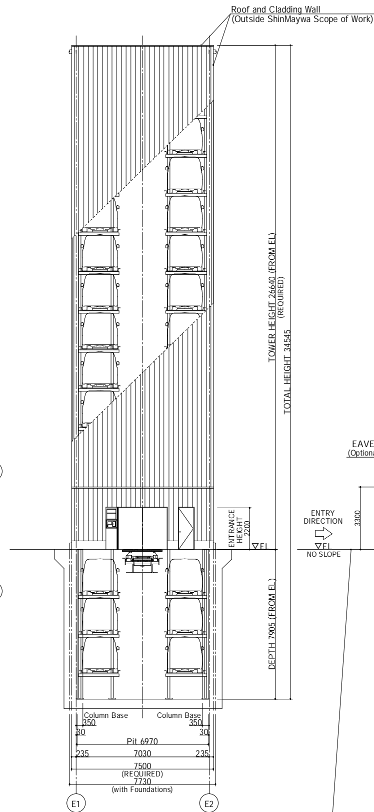
A-A SECTION S = 1/100
