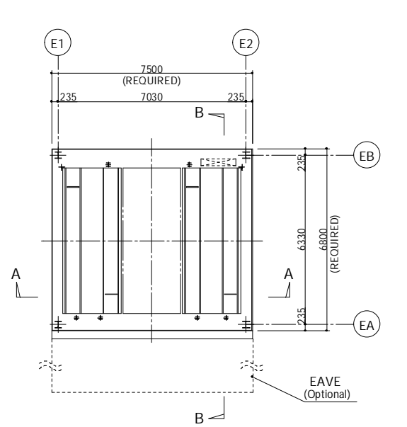
UPPER FLOOR PLAN S = 1/100
