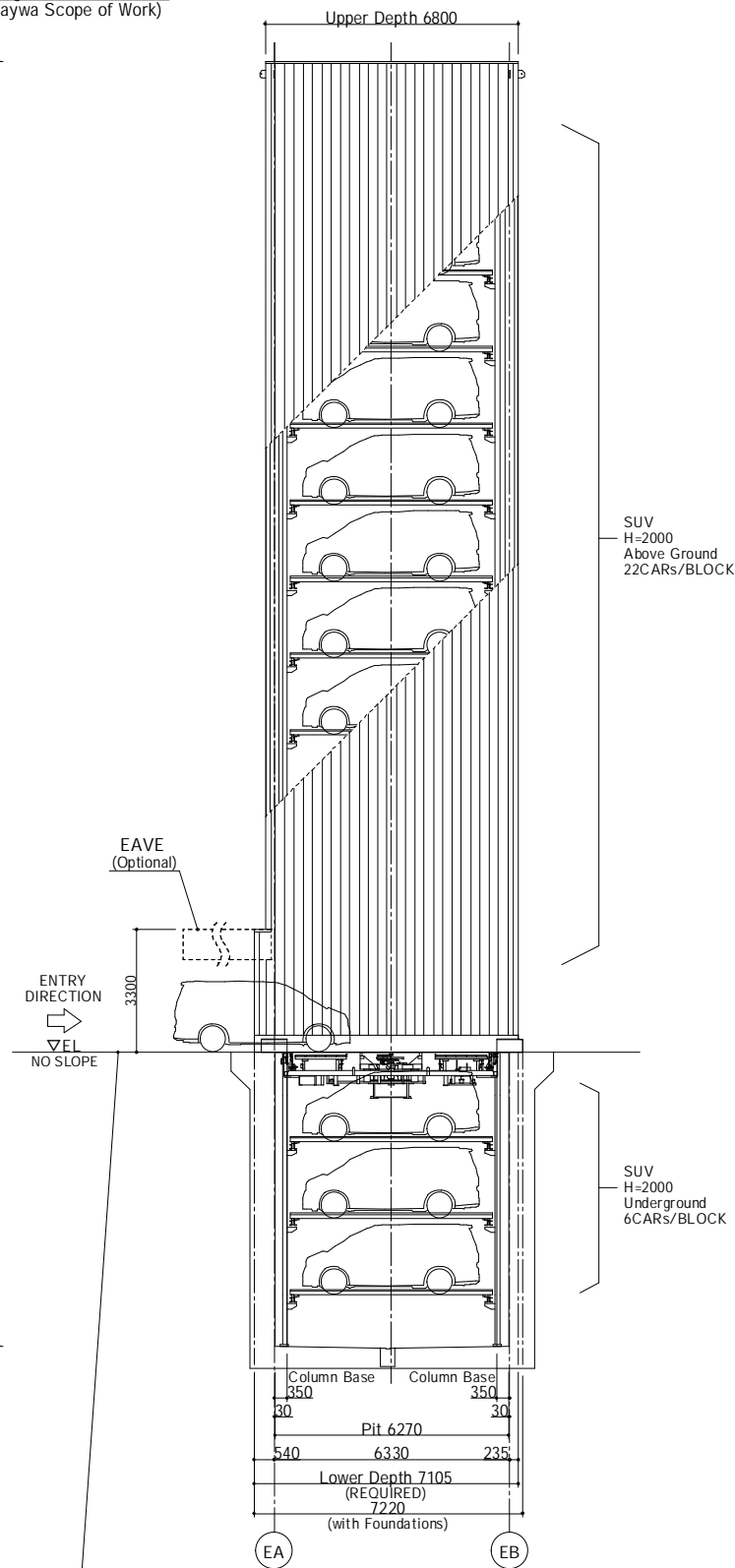
B-B SECTION S = 1/100
