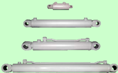
Cylinder for garbage collecting truck
